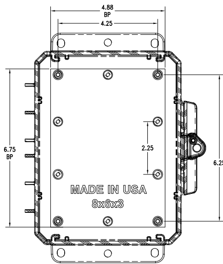
SECTION C-C
