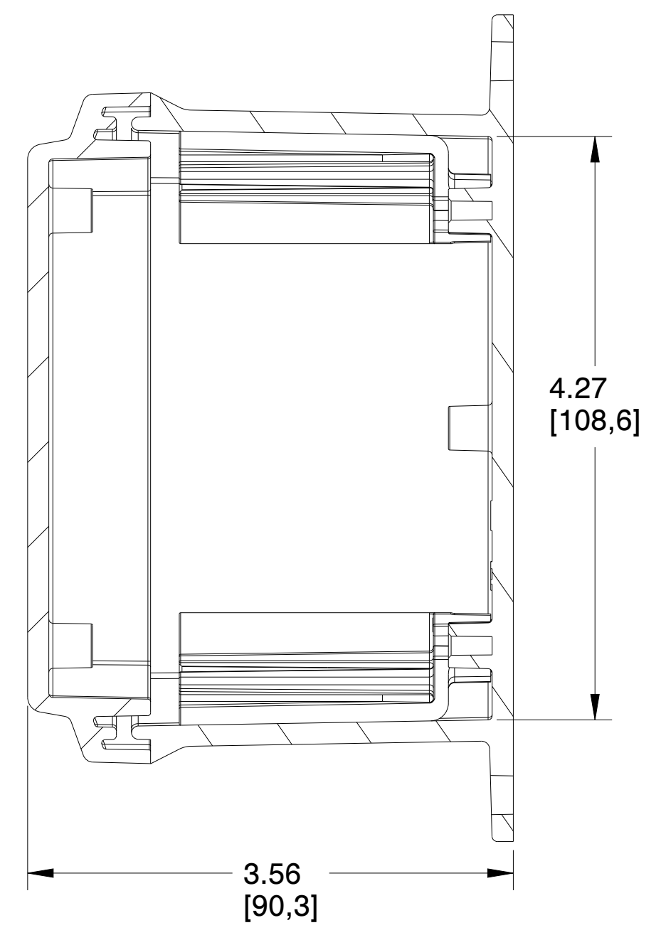
SECTION B-B
