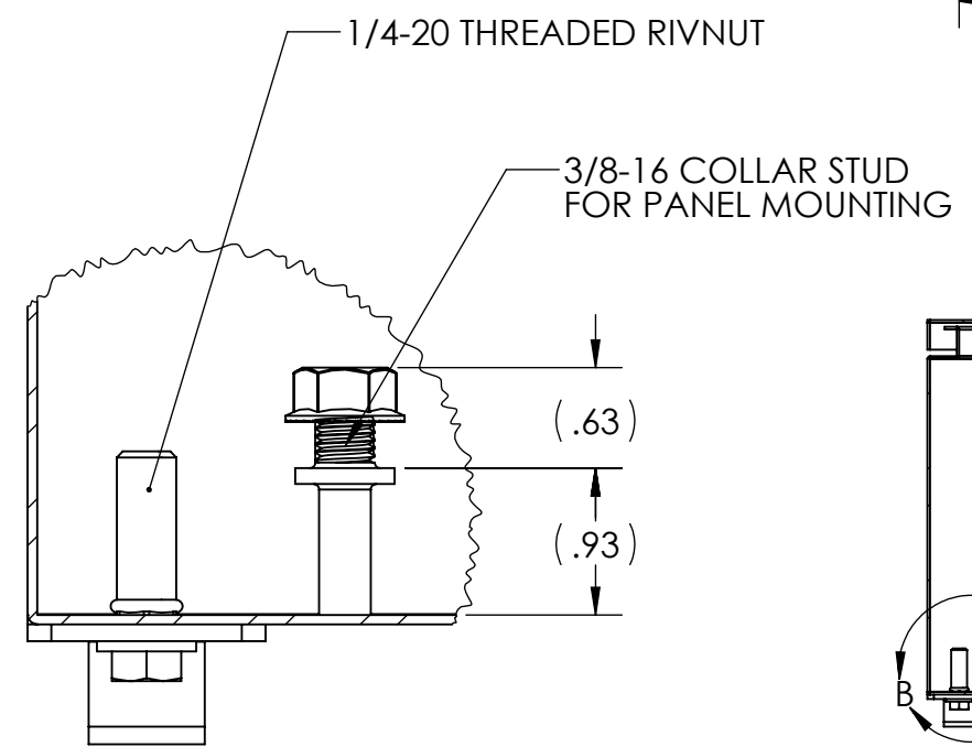
DETAIL B SCALE 3 : 4
