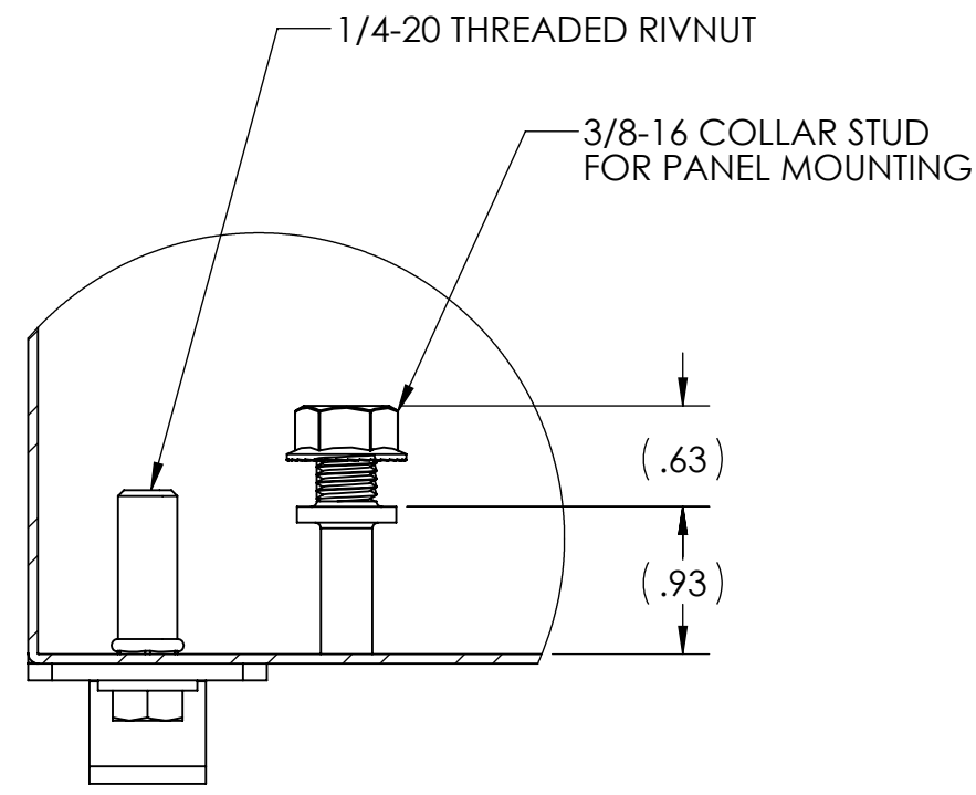
DETAIL B SCALE 3 : 4
